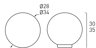
Model. PPL5 ABS
