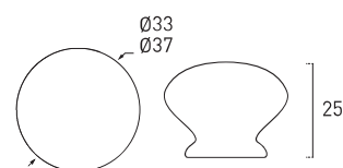
Model. PPL6 ABS
