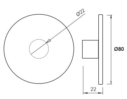
Model. PPL8 ABS
