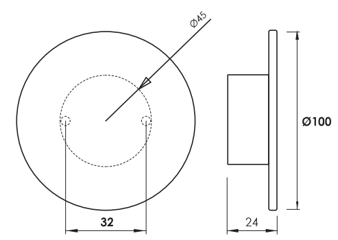
Model. PPL14 ABS
